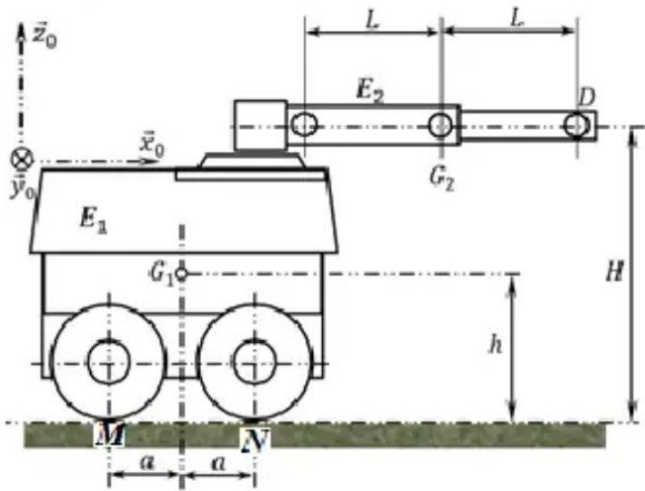
Figure 14 : manipulateur \gamma = 0 et \beta = 0
