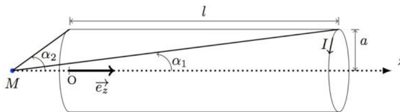
Figure 2.1 : bobine
