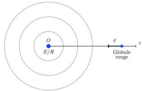
Figure 1 : effet Doppler
