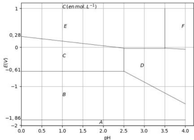
Figure 2: Diagramme E(\text{pH}) de l'uranium
