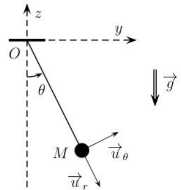
FIGURE 1 – Pendule simple.
