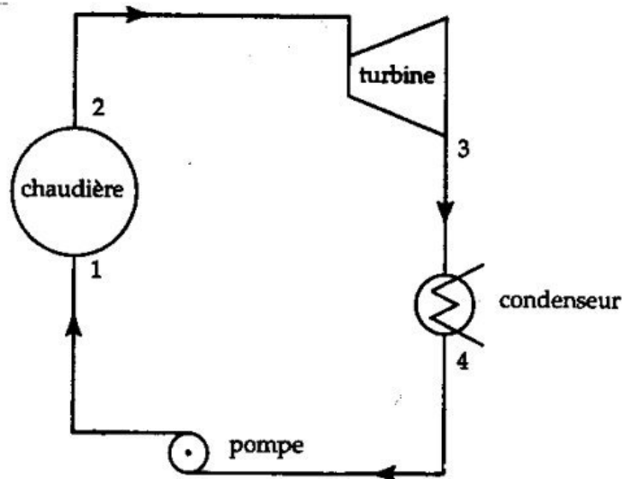
Figure 7: Cycle de RANKINE.
