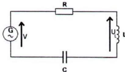
FIGURE 1: circuit RLC
