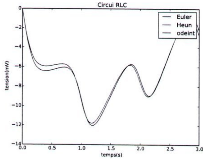
FIGURE 1: circuit RLC
