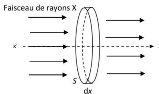
Figure 4 – Absorption de rayons X
