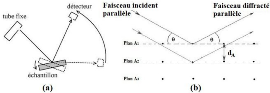
Figure 6 – Dispositif d'étude de diffraction X
