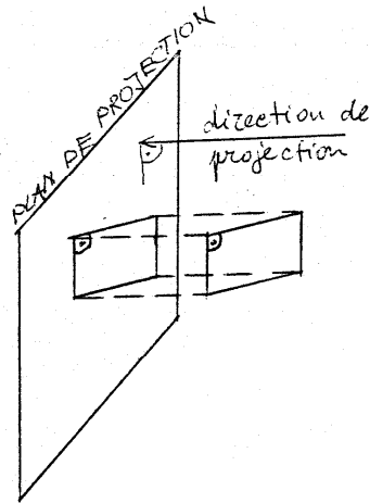
projection orthogonale
